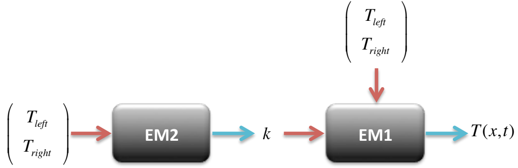
Figure 5 – Heat Conduction Ensemble-Model connections in chain of evaluations
