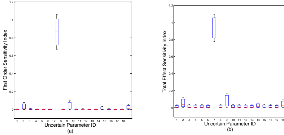
Figure 5. Quantified BBC Sensitivity Indices with respect to Caesium-137
