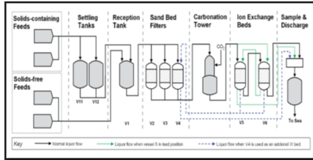
Fig 1. SIXEP Process Diagram [8]
