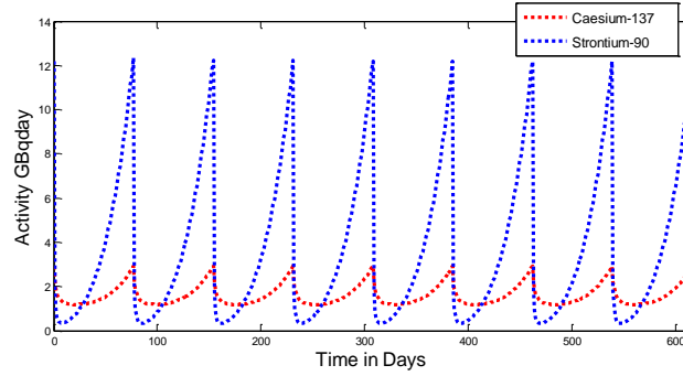
Fig. 2. Deterministic Simulation from the SIXEP Model
