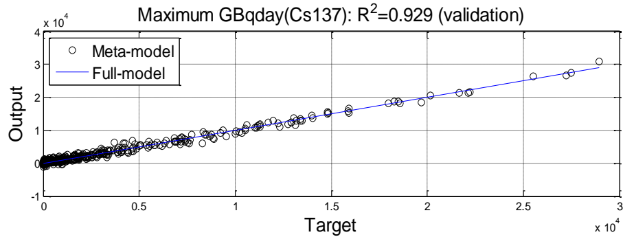
Figure 3. Performance of ANN mapping Caesium-137
