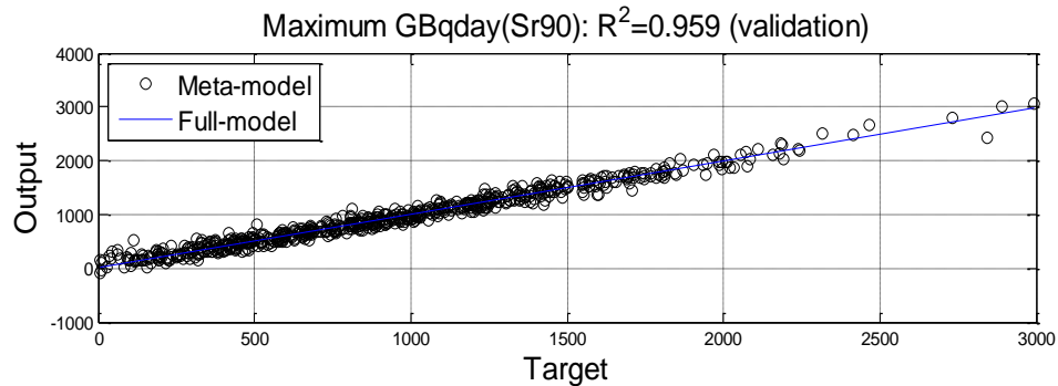
Figure 4. Performance of ANN mapping Strontium-90
