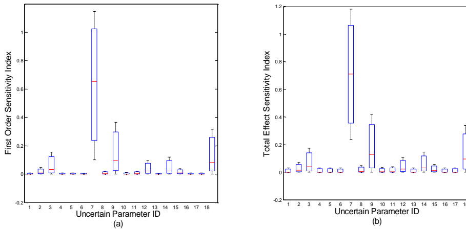
Figure 6. Quantified BBC Sensitivity Indices with respect to Strontium-90
